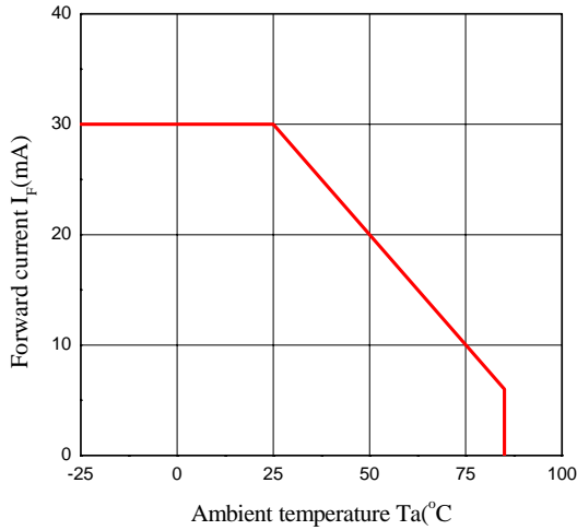
Forward Current vs Derating Curve
